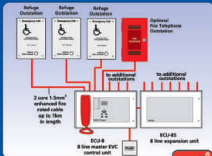
A TYPICAL WIRING SCHEMATIC
